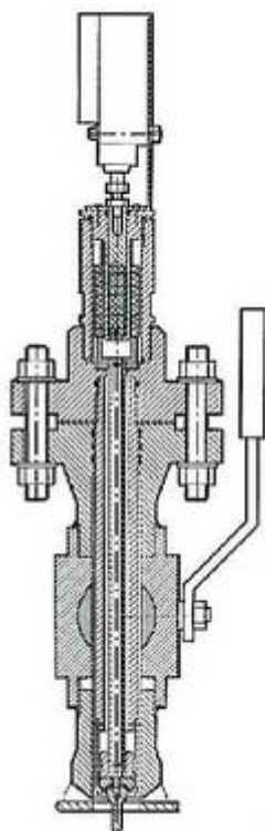
VALVED ELECTRICAL DIRECT MOUNTED MODEL 'EVW'
