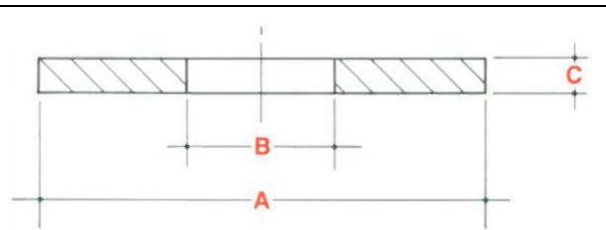
General dimensions
