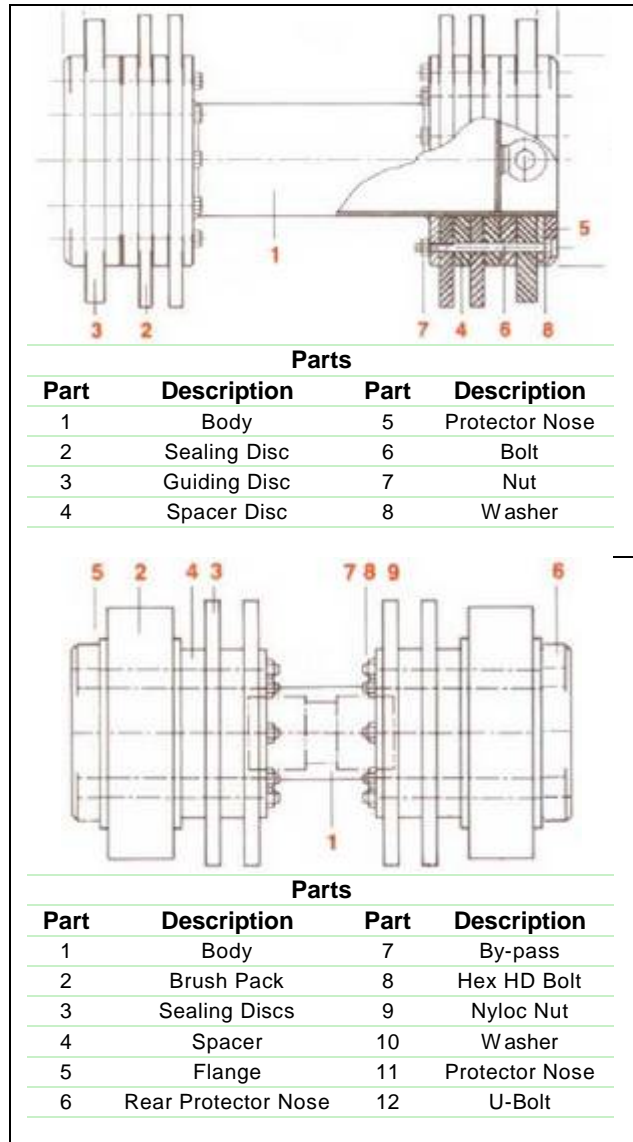
IP. HS HI-SEAL BI-DIRECTIONAL PIG 2" thro 48"
