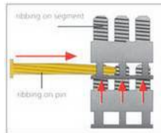
Drawing 1 : the inside view.
