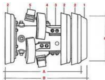
IP.UG2 - 16" thro 48" CLEANING PIG
