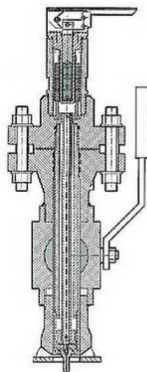
VALVED MECHANICAL DIRECT MOUNTED MODEL 'MWW'
