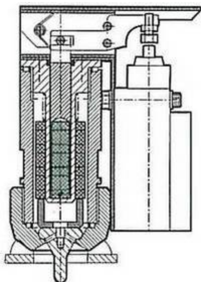
COMBINED MECHANICAL-ELECTRICAL DIRECT MOUNTED MODEL 'CW'
