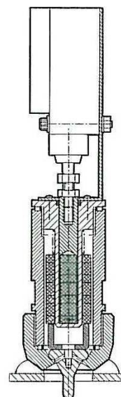
ELECTRICAL DIRECT MOUNTED MODEL 'EW'
